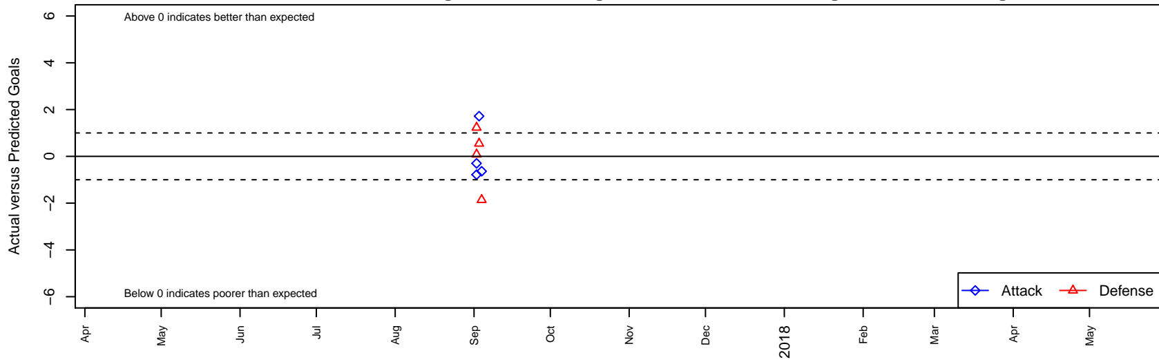
Delta Coastal Selects B03 Dots are actual minus expected GF (blue circles) and GA (red triangles). Blue line is smoothed change in attack strength. Red is smoothed change in defense strength.
